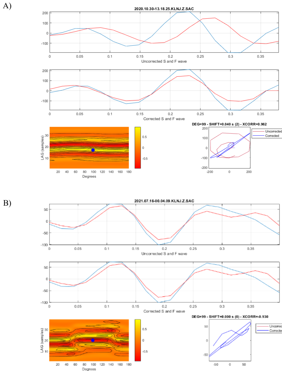
Figure 5. A) An example of the output of the anisomat+ code, where the ( \delta t ) and ( \phi ) have been obtained. b) An example of a null output in which the S wave is not splitted and shows the linear particle motion.
