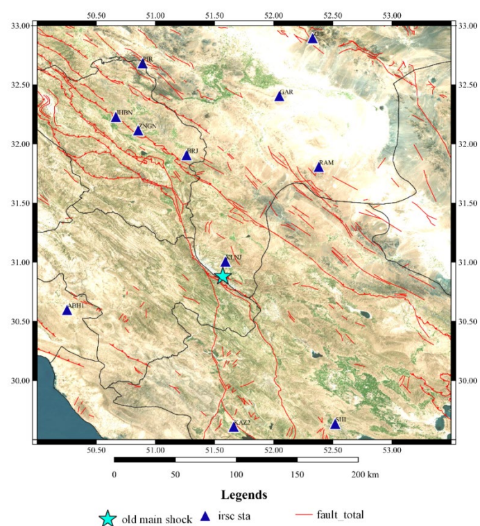
Sisakht Earthquak(1399/11/29, Mn=5.4)
