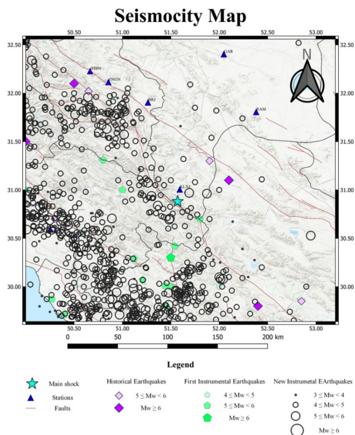
Figure 2. Seismicity of the region of this study.
